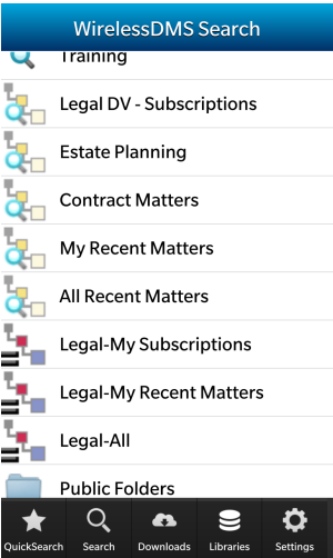
BlackBerry 10 UI
